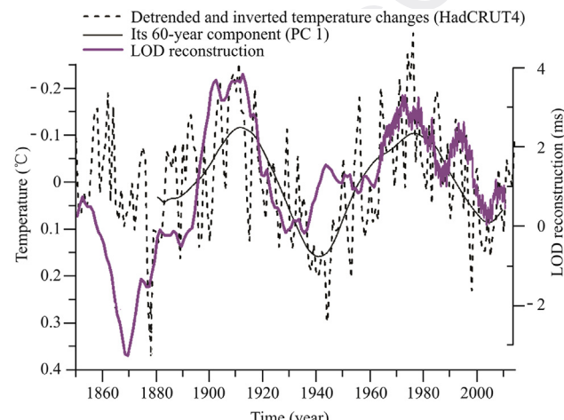
Fig. 3 – Long-term LOD compared with detrended and inverted temperature changes.
