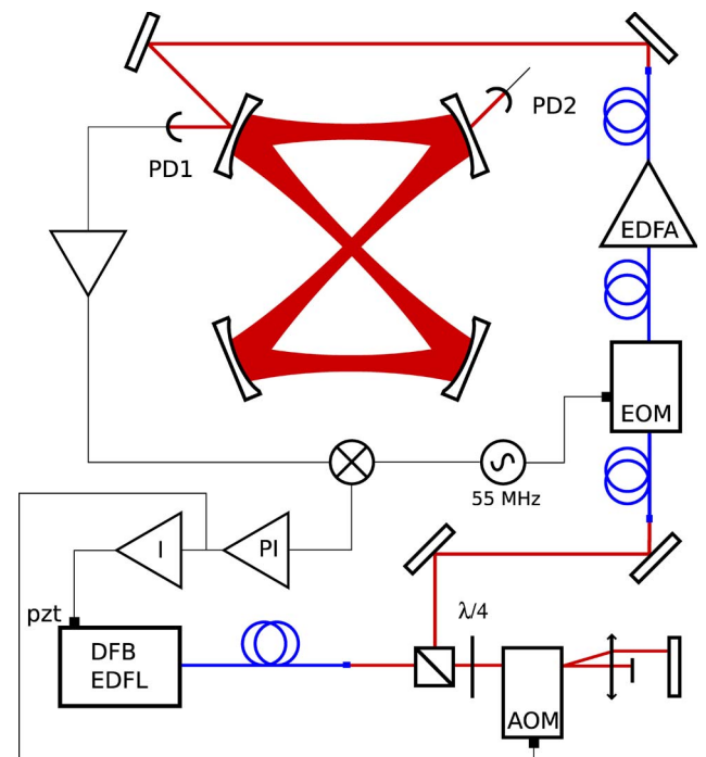
Fig. 1. (Color online) Frequency stabilization setup to lock the DFB EDFL to a transverse mode of the folded optical cavity. The fibered and the free-space optical path are shown in blue and red; the electronic connections are shown in black.
