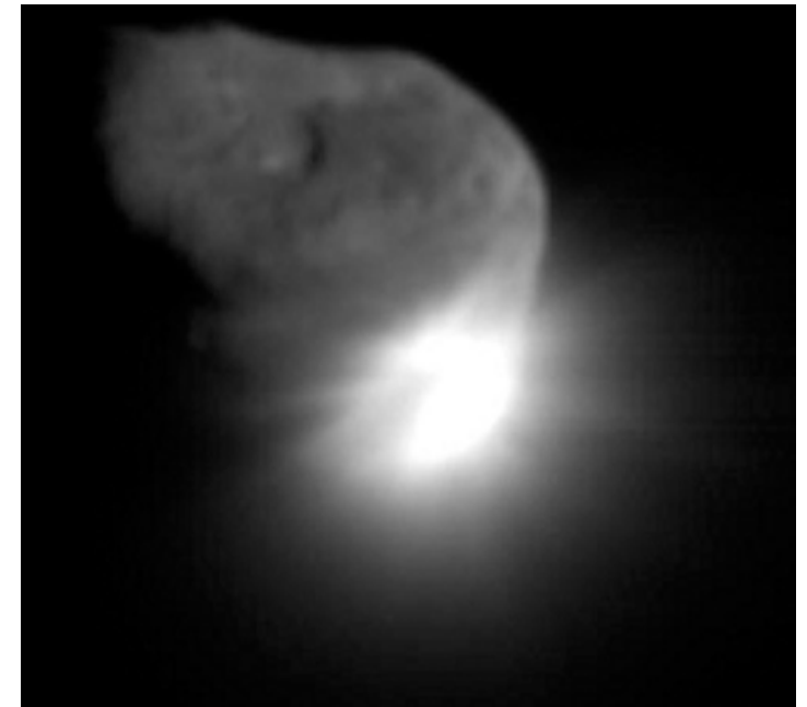
Deep Impact/Tempel 1)
