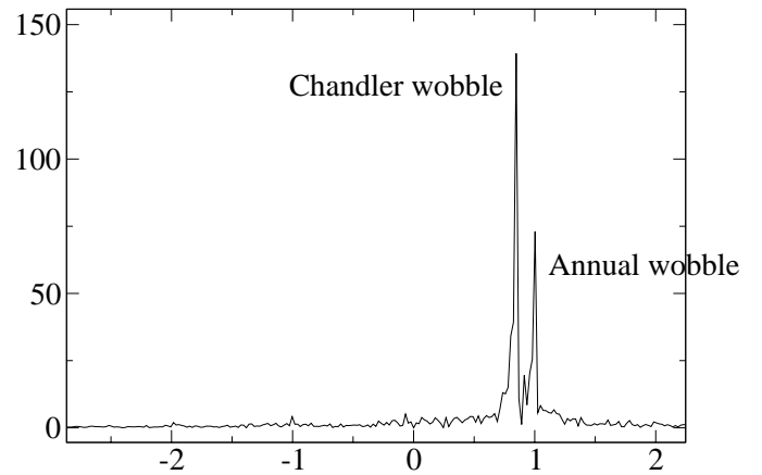
Fig. 3. Complex spectrum of polar motion (Fast Fourier Transform) over the total duration of the IERS C04 series (1962–2002), amplitudes are in mas, frequencies are in cycles per year (cpy).
